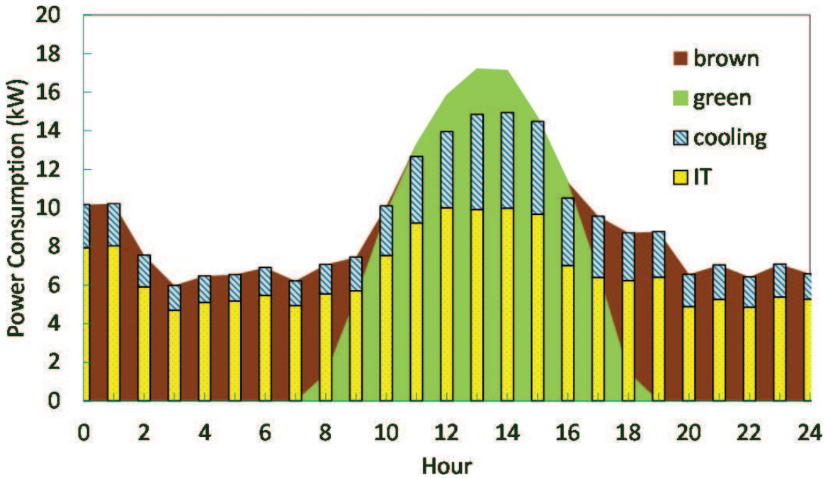
Figure 8. Power consumption details under JOP strategy.
