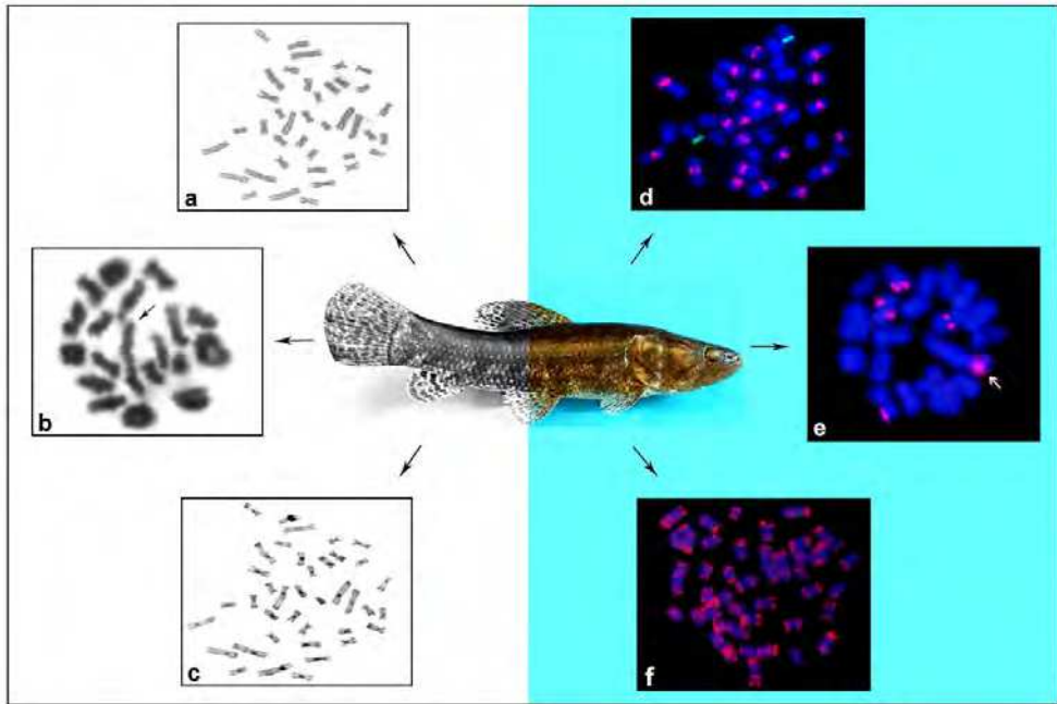
Fig. 1. Conventional (a, b and c) x molecular (d, e, and f) cytogenetic analyses in chromosomes of males of the karyomorph D of the fish Hoplias malabaricus ( 2n = 39, X_1X_2Y sex chromosomes) highlighting the transition from the "black-and-white" to the "color" era. Giemsa-stained mitotic chromosomes (a) and diakinesis/metaphase I meiotic cell (b); C-banded (c); 5S rDNA (green) and satellite 5SHindIII-DNA (red) hybridized to mitotic chromosomes (d); diakinesis/metaphase I meiotic cell displaying 18S rDNA sites (red) in the synapsed chromosomes (e); simple sequence repeat (GA) 15 (red) hybridized to mitotic chromosomes. The arrows indicate the sex trivalent.
