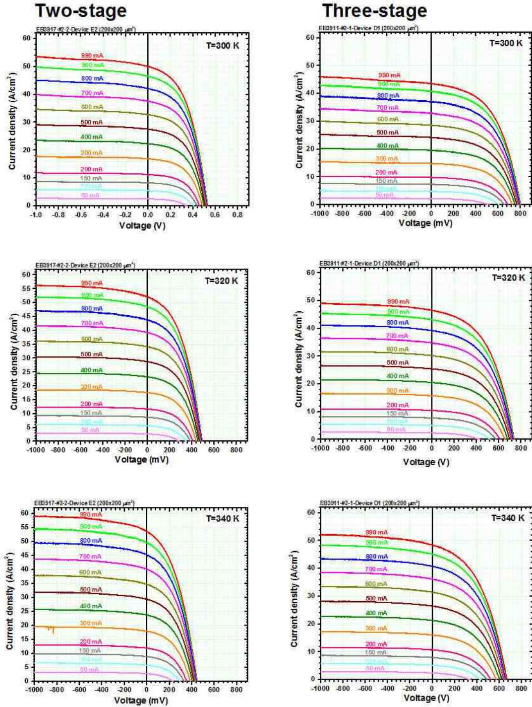
Figure 7-6: J-V curves for representative devices from two- and three-stage ICTPV wafers under different laser illumination levels. The legend above each curve shows the injection current applied to the IC laser. Higher injection currents correspond to higher levels of laser illumination that was incident on TPV cells.
