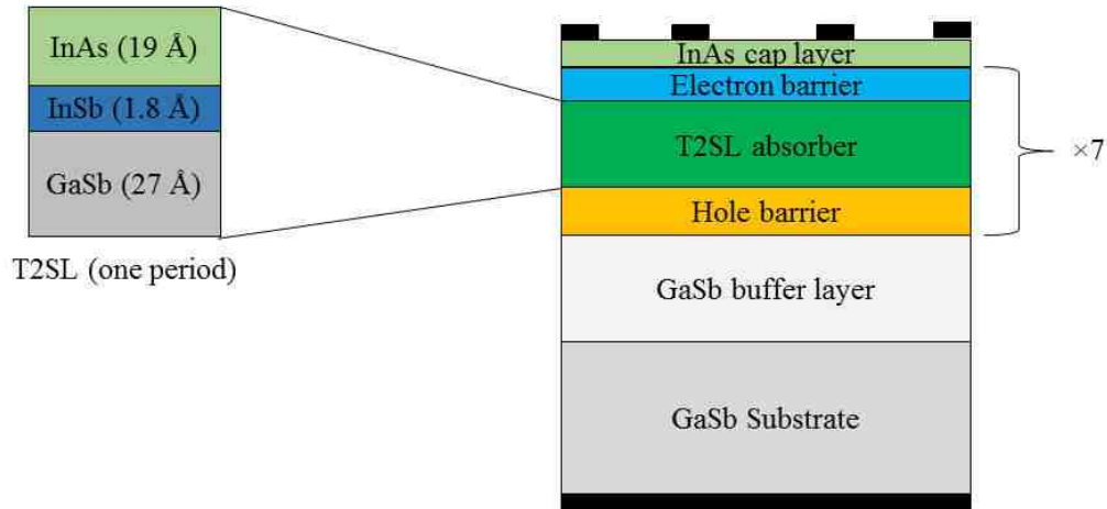
Figure 7-13: Schematic structure of the seven-stage narrow-bandgap ICTPV cells. Absorbers were identical in all stages and had similar absorber thickness of ~158 nm.
