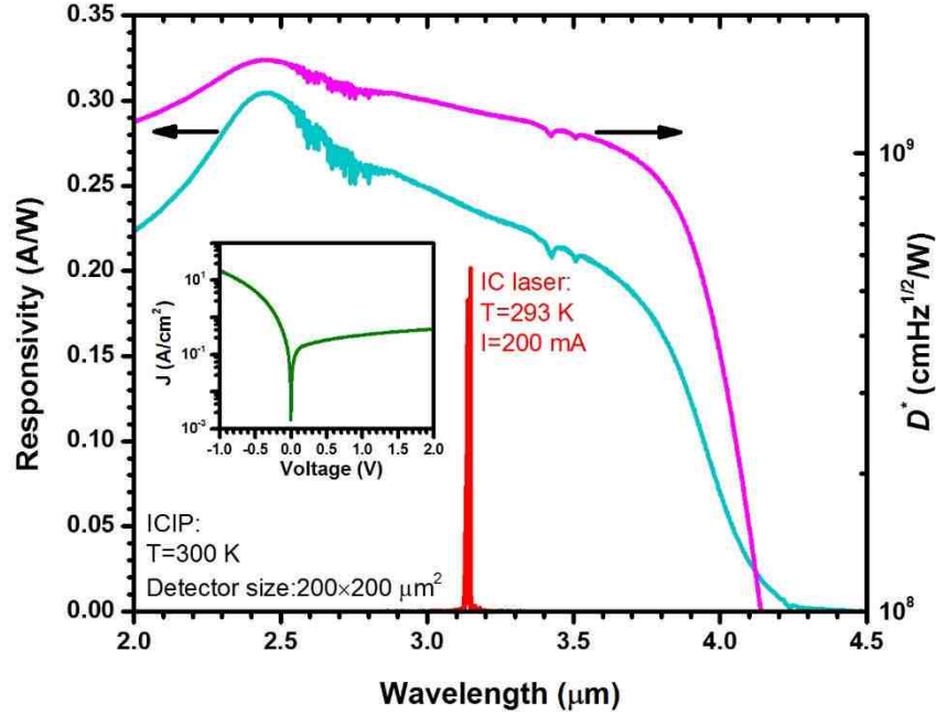
Figure 5-3: Zero-bias responsivity and Johnson-noise-limited detectivity for a 200\times 200\ \mu\text{m}^2 ICIP at 300 K. The IC laser emission spectrum at T=293\ \text{K} , under 200 mA injection, is also displayed. Inset, dark J - V curve for the same ICIP at 300 K.
