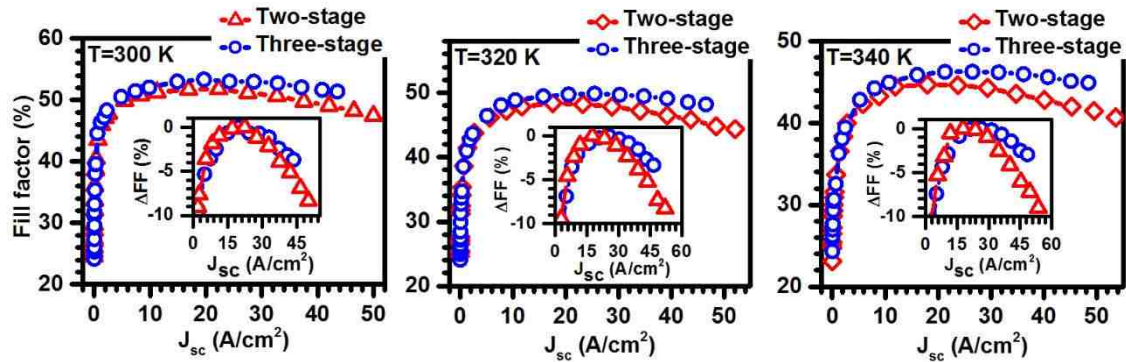
Figure 7-7: Device fill factor vs. J_{sc} for representative 200 \times 200 \mu\text{m}^2 devices from two- and three-stage wafers at T=300-340 K. Insets show \Delta FF for the same devices at different short-circuit currents. Two-stage device exhibited sharper decrease (compared to the three-stage device) in fill factor at high illumination levels.
