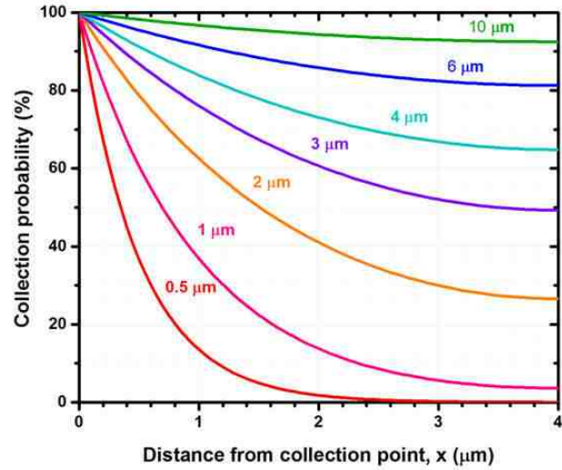
Figure 2-8: Collection probability for minority carriers ( i.e. , electrons) vs. their distance from the collection point (hole barrier) in a hypothetical photodetector with a 4 μm-thick absorber. Provided numbers on each curve denote the assumed minority carrier diffusion lengths. Minority carrier diffusion lengths below 1 μm are realistic assumptions for T2SL photodetectors at high temperatures as discussed in the following chapters. The left side panel shows the simplified structure of one stage in an ICIP.
