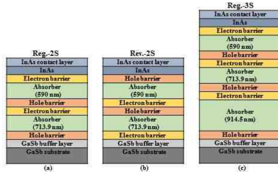
Figure 3-1: Device structure for the ICIPs: (a) regular-illumination configured two-stage (Reg.-2S), (b) reversed-illumination configured two-stage (Rev.-2S); and (c) regular-illumination configured three-stage (Reg.-3S). Device illumination was from the top in all of these detectors.
