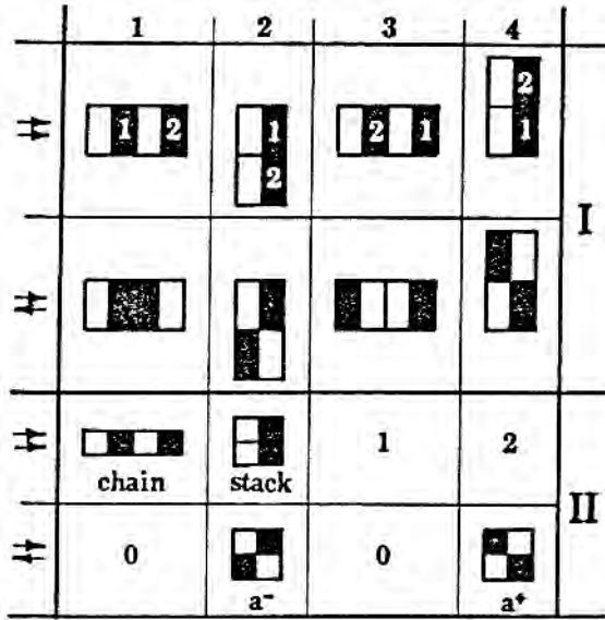
FIGURE 7. Elementary tessellations.
