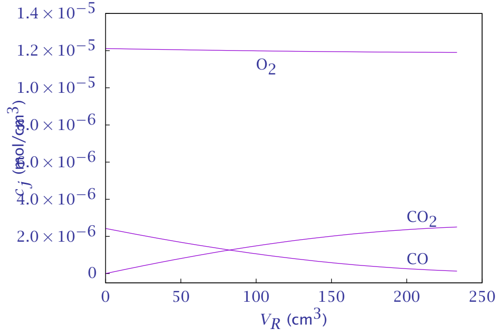
Figure 22: Molar concentrations versus reactor volume.
