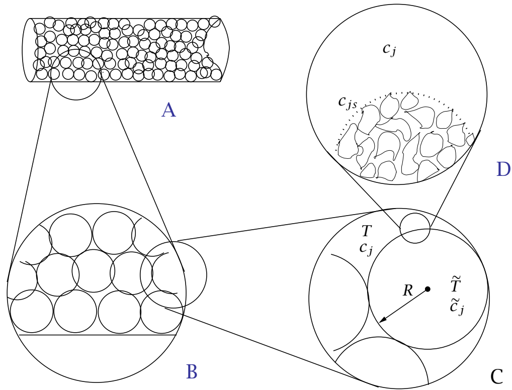
Figure 2: Expanded views of a fixed-bed reactor.
