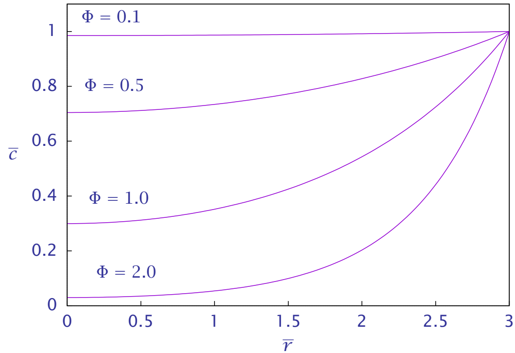
Figure 4: Dimensionless concentration versus dimensionless radial position for different values of the Thiele modulus.
