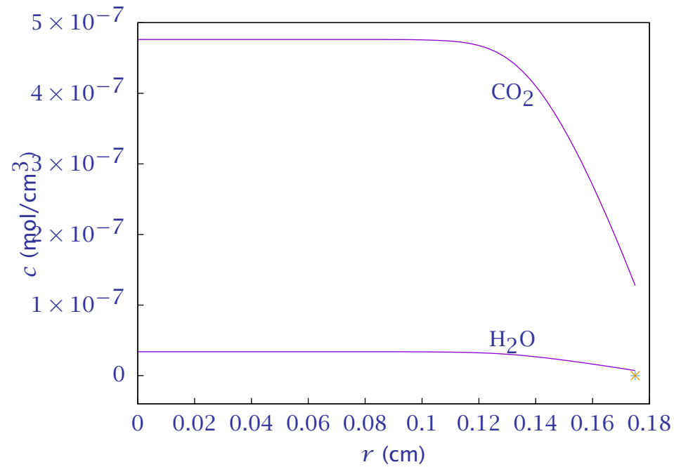
Figure 19: Concentration profiles of the products; fluid concentration of CO 2 (×), H 2 O (+).
