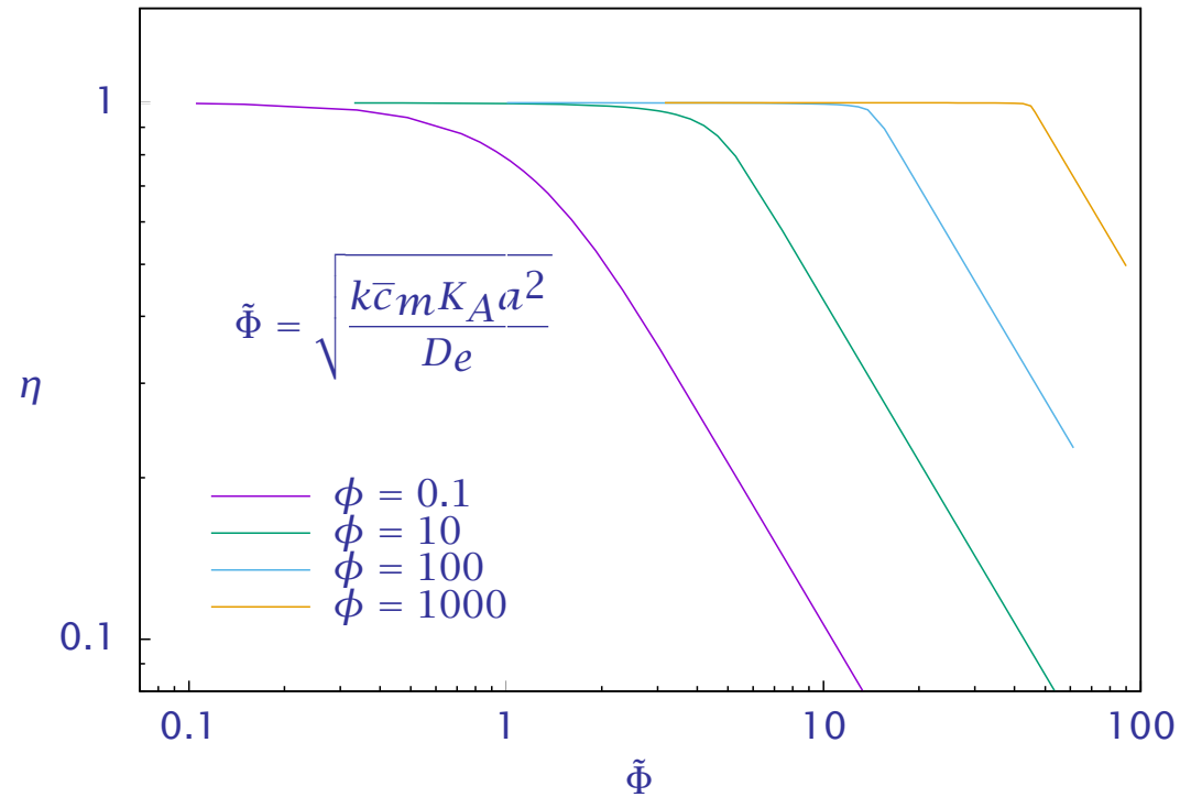
Figure 11: Effectiveness factor versus an inappropriate Thiele modulus in a slab; Høugen-Watson kinetics.
