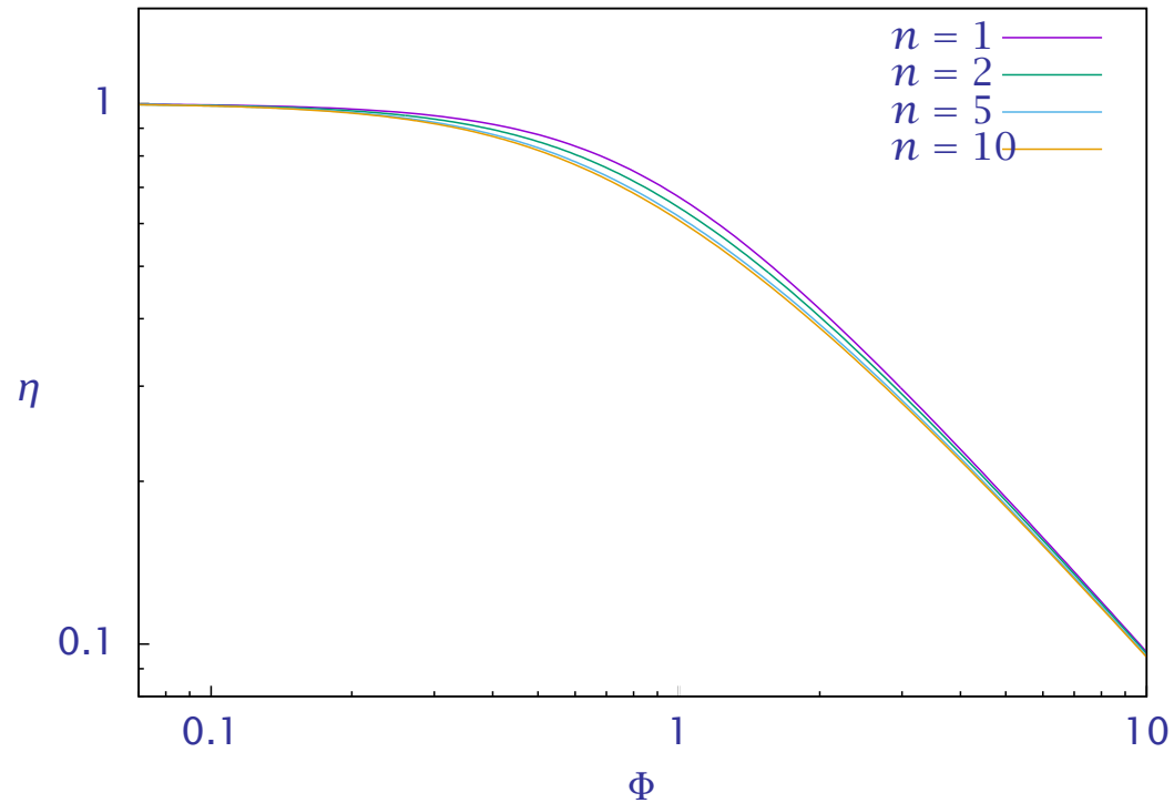
Figure 8: Effectiveness factor versus Thiele modulus in a spherical pellet; reaction orders greater than unity.
