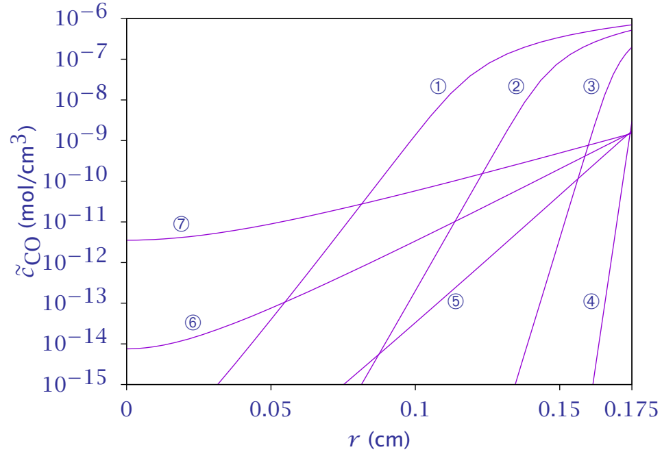
Figure 27: Pellet CO profiles at several reactor positions.
