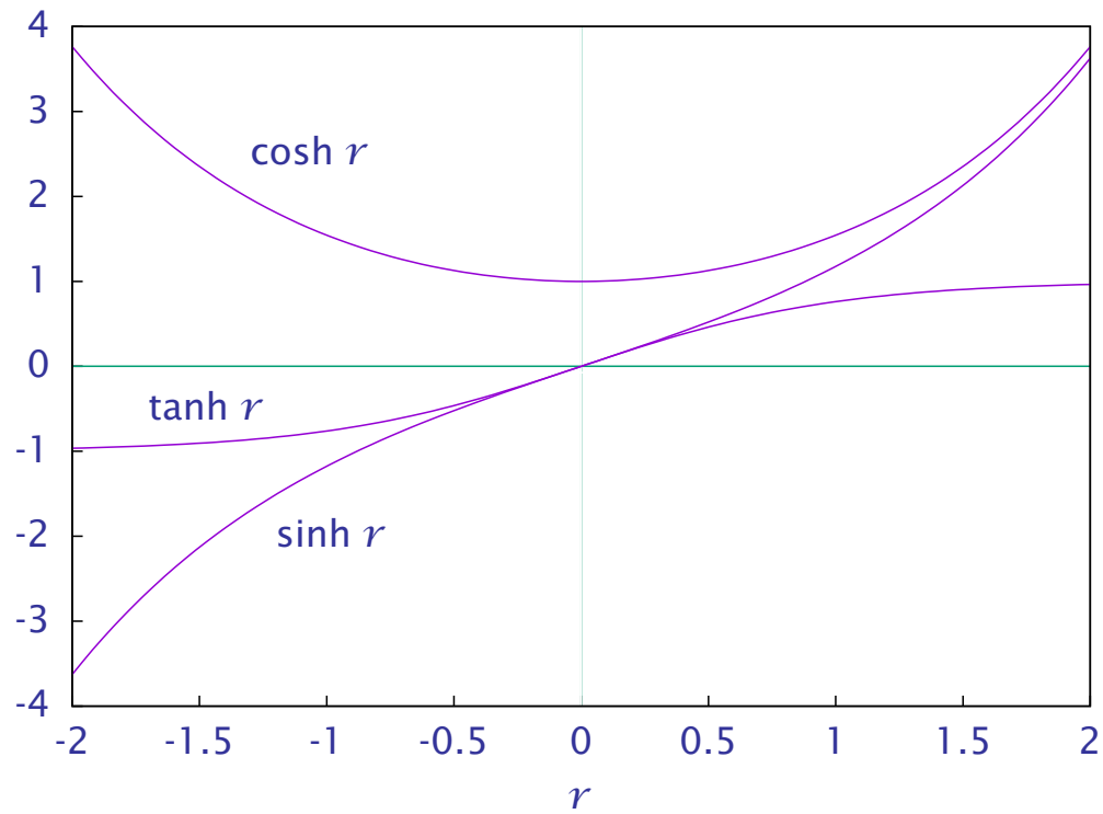
Figure 3: Hyperbolic trigonometric functions \sinh , \cosh and \tanh .
