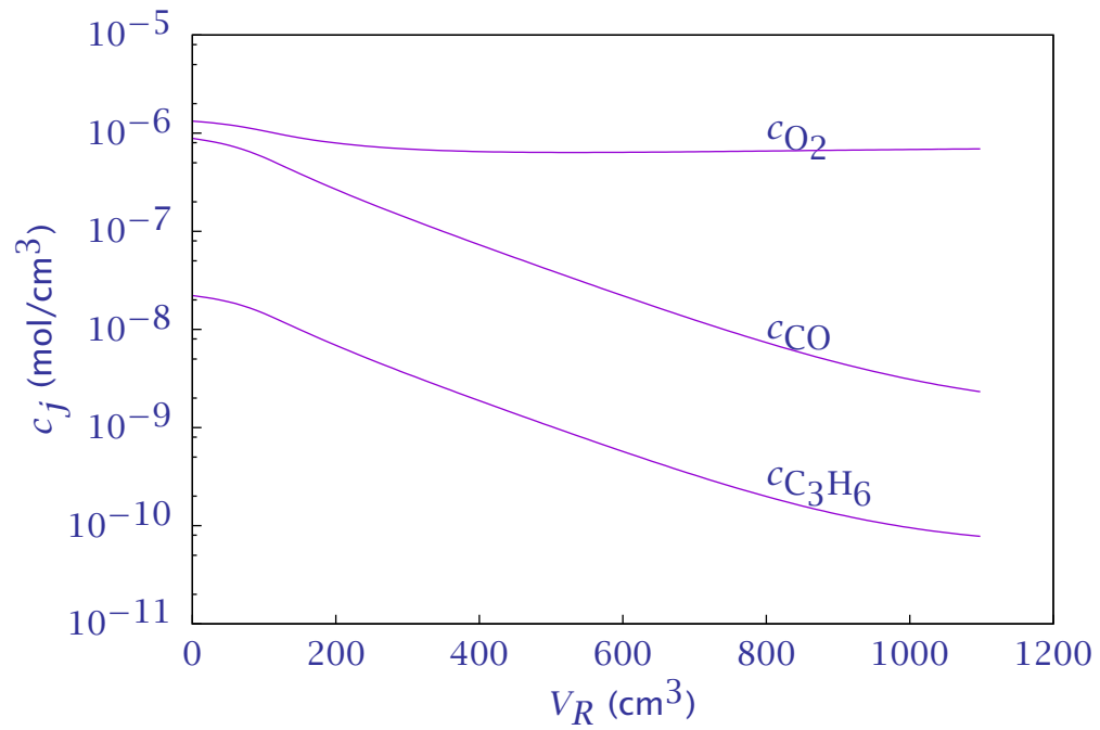
Figure 24: Fluid molar concentrations versus reactor volume.
