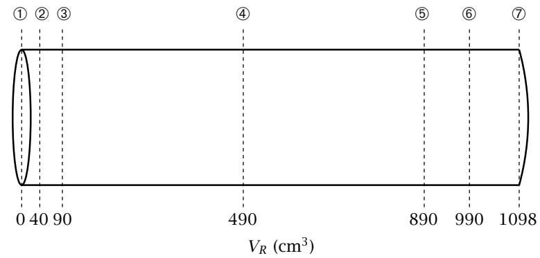
Figure 26: Reactor positions for pellet profiles.
