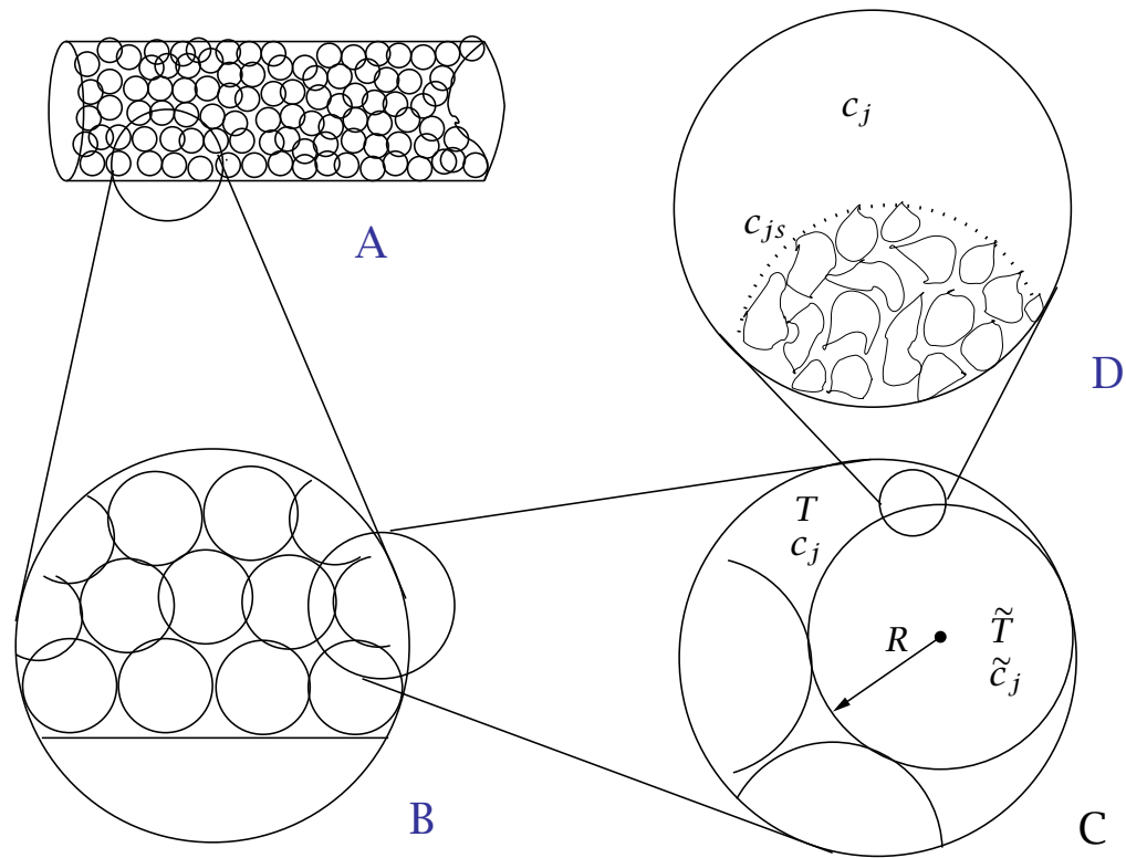
Figure 1: Expanded views of a fixed-bed reactor.
