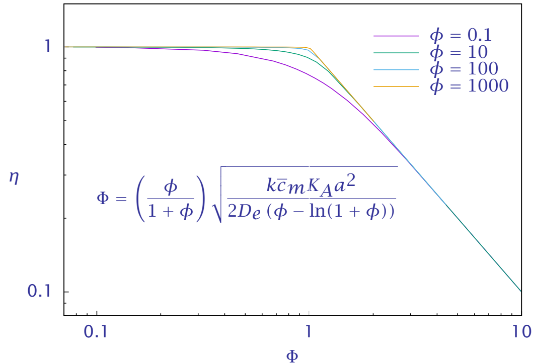
Figure 12: Effectiveness factor versus appropriate Thiele modulus in a slab; Hougen-Watson kinetics.
