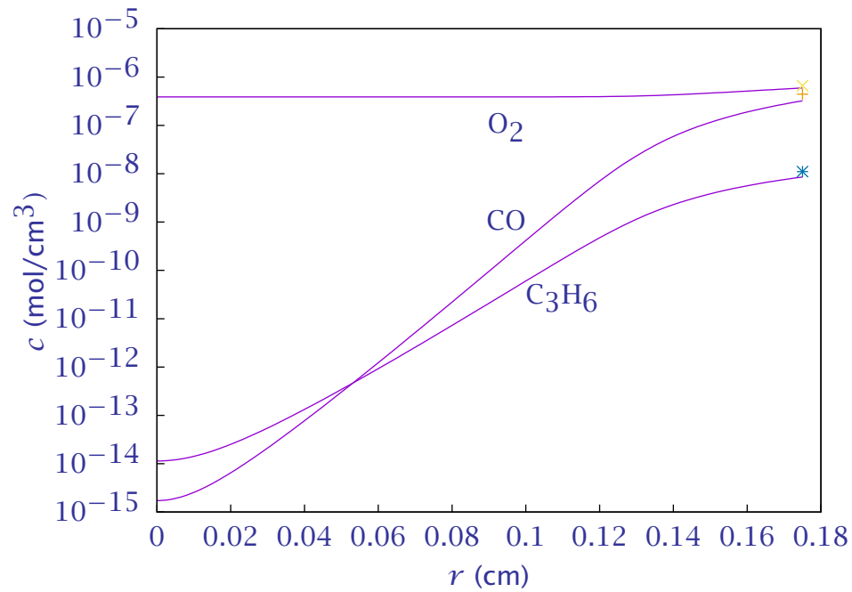
Figure 18: Concentration profiles of reactants (log scale); fluid concentration of O_2 ( \times ), CO ( + ), C_3H_6 ( * ).
