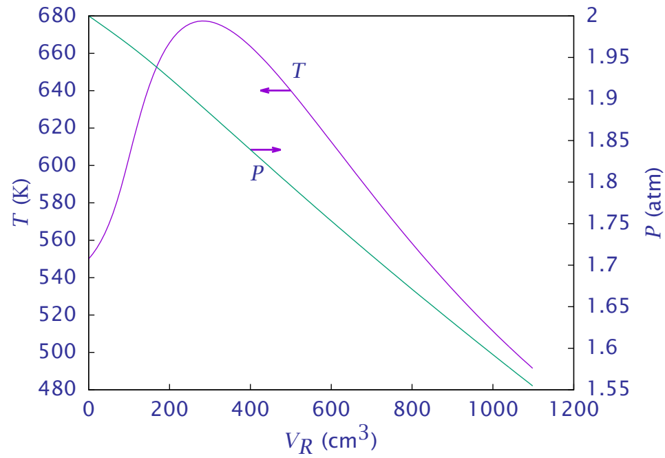
Figure 25: Fluid temperature and pressure versus reactor volume.
