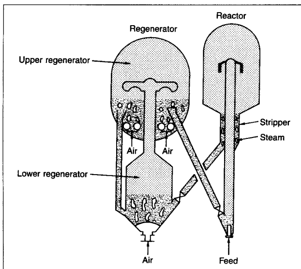
Figure 3-6. Typical FCC reactor/regeneration. 26
