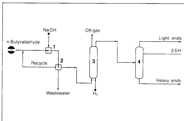
Figure 8-6. The Hoechst AG process for producing 2-ethylhexanol from n -butyraldehyde: 22 (1) Aldol condensation reactor, (2) separation (organic phase from liquid phase), (3) hydrogenation reactor, (4) distillation column.
