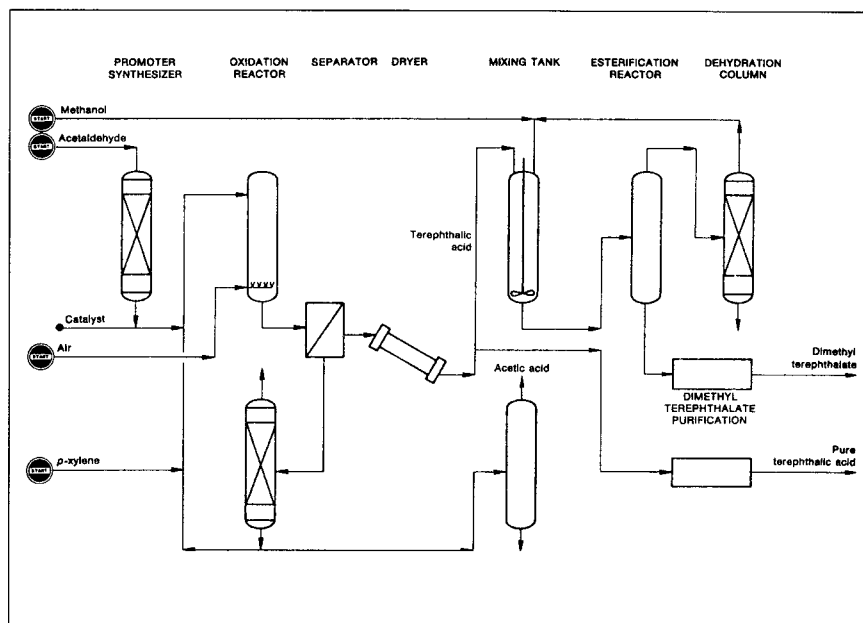
Figure 12-9. The Inventa AG Process for producing polyethylene-terephthalate. 47
